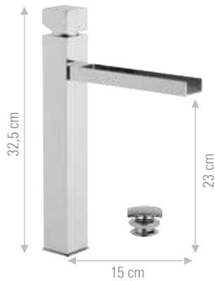
CW607 Monocomando lavabo alto con bocca a cascata, con scarico click-clack. High basin mixer with waterfall spout, with click-clack waste.
