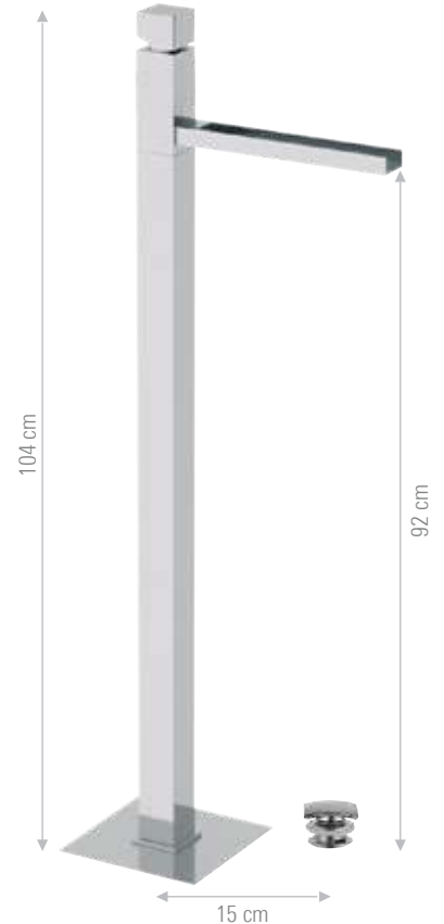
CW688 Miscelatore monocomando lavabo da pavimento con click-clack e troppo pieno. Single-lever mixer floor mounting with click-clack and overflow.
